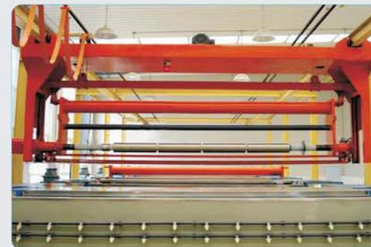
← Plating line for gravure platemaking
